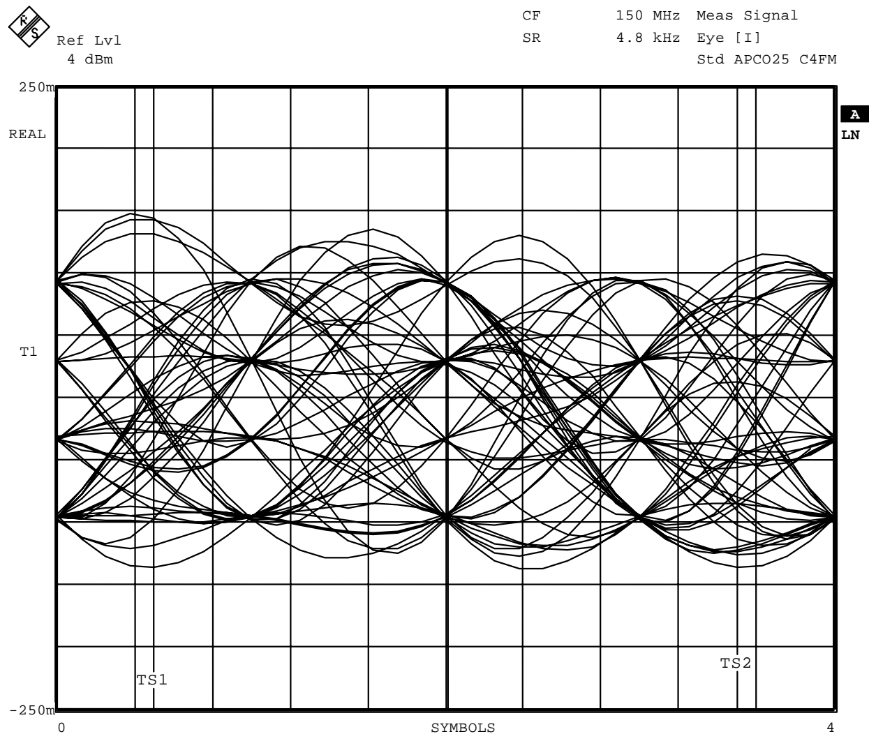
Figure 7 C4FM PRBS Waveform (eye diagram)
