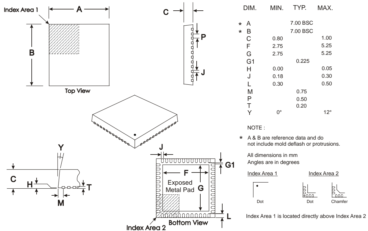
Figure 21 Mechanical Outline of 48-pin VQFN (Q3)
