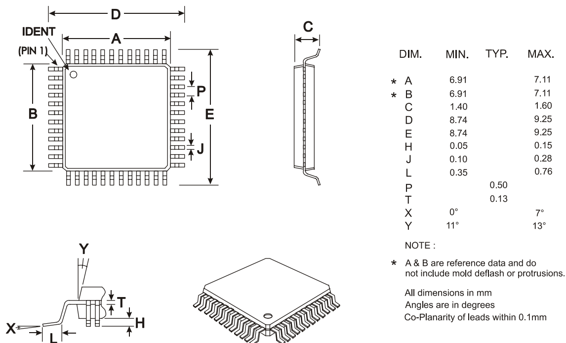
Figure 22 Mechanical Outline of 48-pin LQFP (L4)
